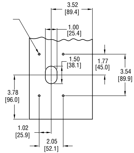
LATERAL OUTPUT PORT (DUAL OUTPUT PORT INSTRUMENTS ONLY)
