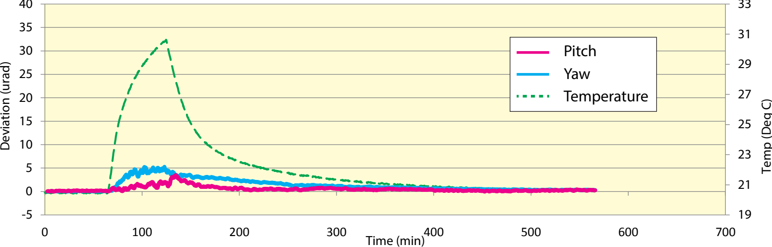
Suprema® with ZeroDrift™ Thermal Drift Compensation
