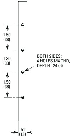
VIEW A
