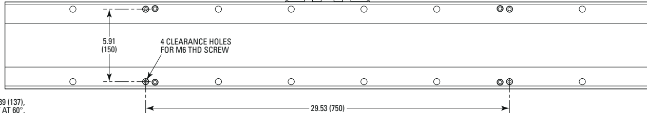
VIEW A
