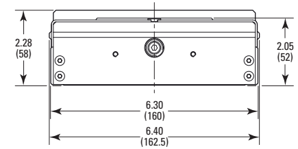
-VIEW F-
