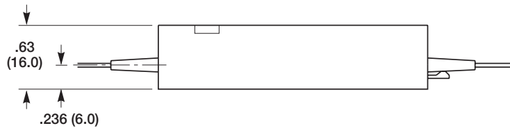
1x2 fiber-optic prism switch
