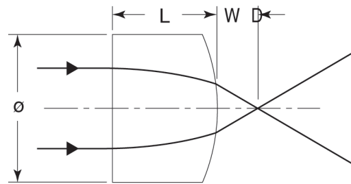
0.22 Pitch, Plano-Convex
