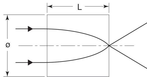
0.25 Pitch, Plano-Plano
