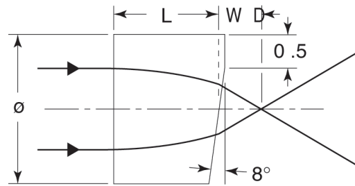
0.23 Pitch, Plano-Angled
