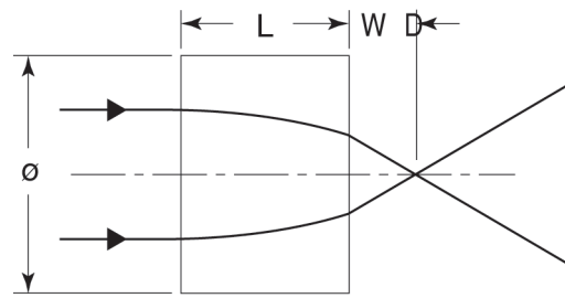
0.23 Pitch, Plano-Plano
