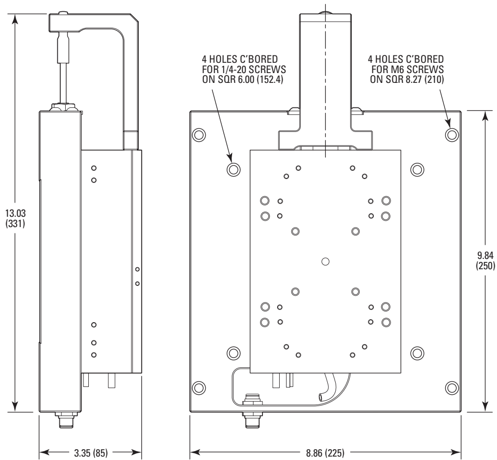
MODEL SHOWN: XMS100V DIMENSIONS IN INCHES (AND MILLIMETERS)
