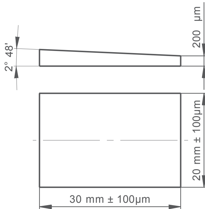
Ultra thin wedge - conceptual drawing.
