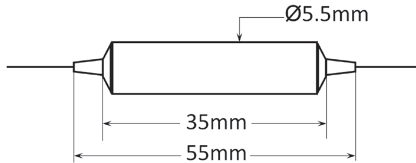
Pigtailed, FC Connector
