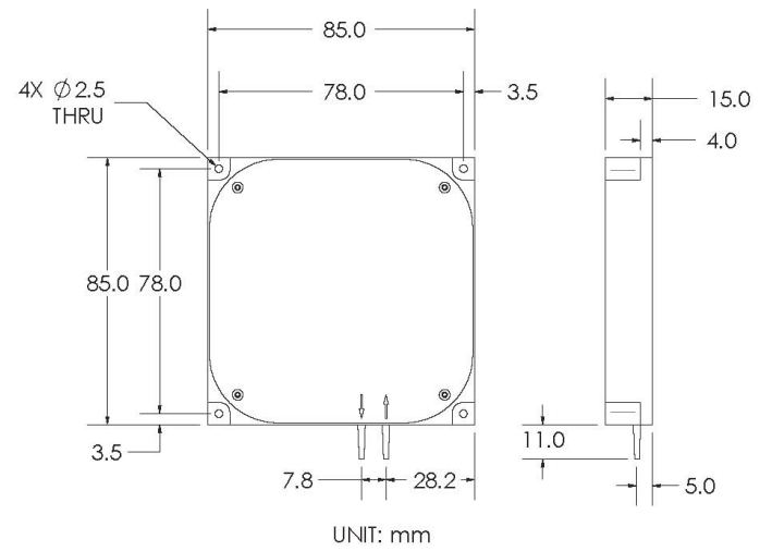
Standard package for DEP-003
