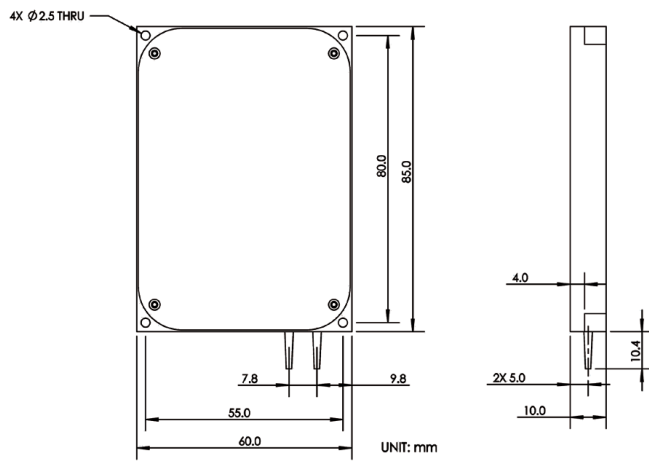
Alternate smaller package for depolarizers with small coherence lengths
