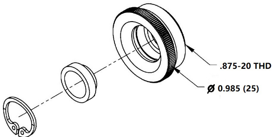
MODEL NO. 910P-MNT
