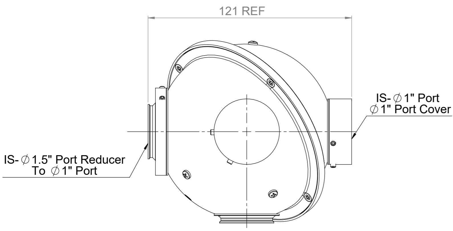
Top View
