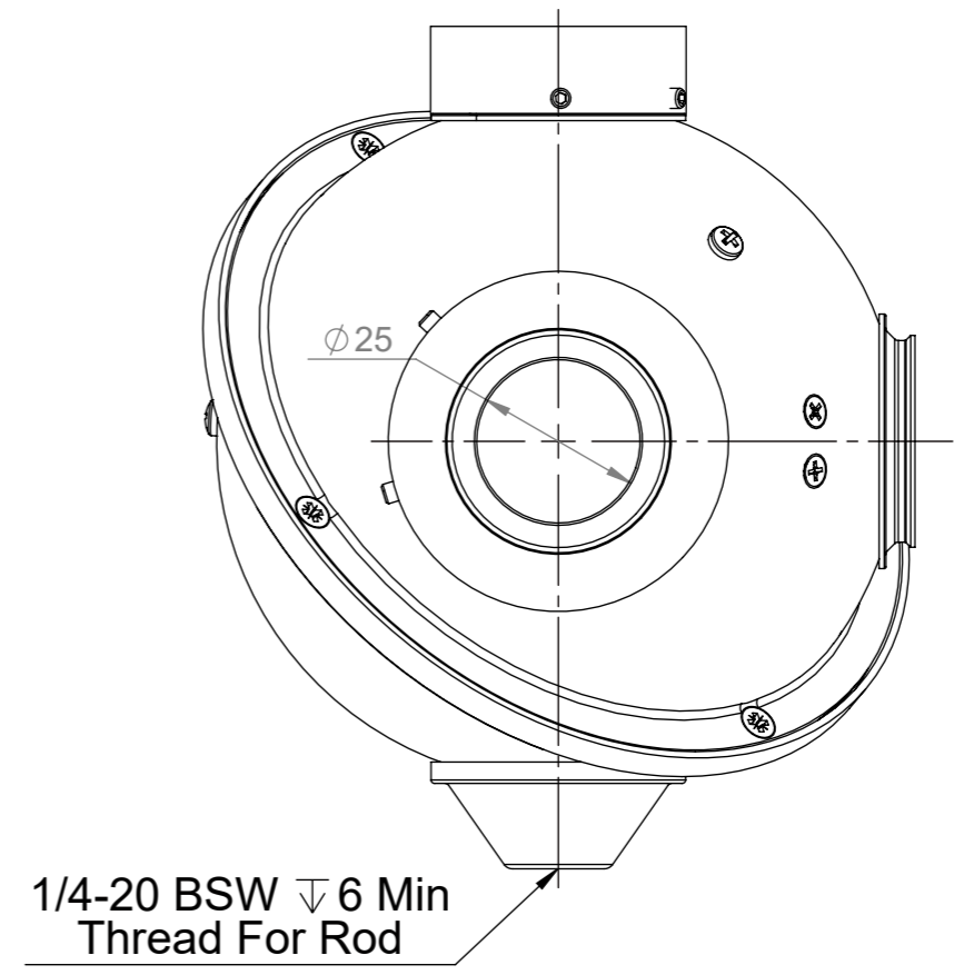
Side View
