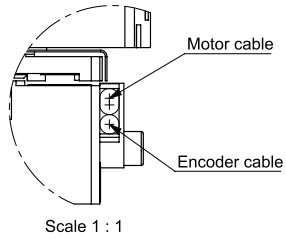
Cable placement in the clamp
