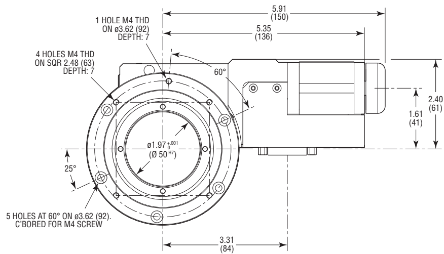
BOTTOM VIEW OF THE RVS80PP
