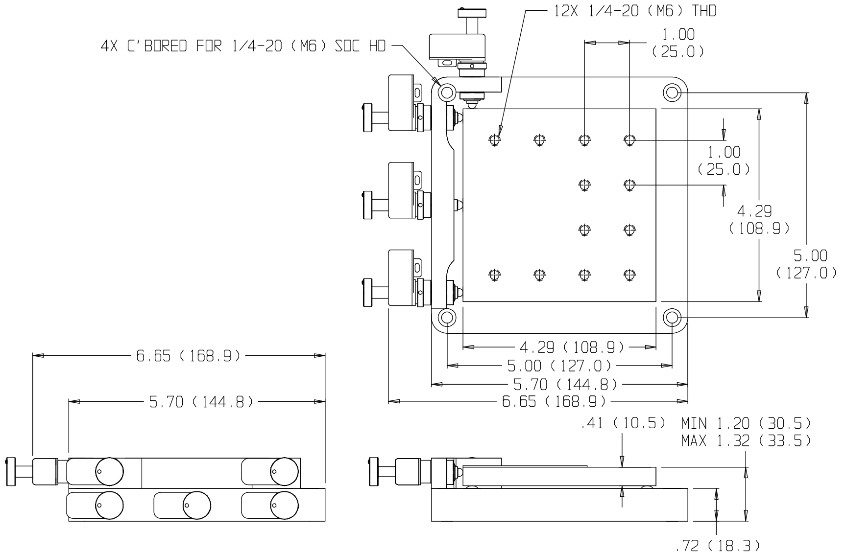
8095(M) MOTORIZED 6-AXIS STAGE
