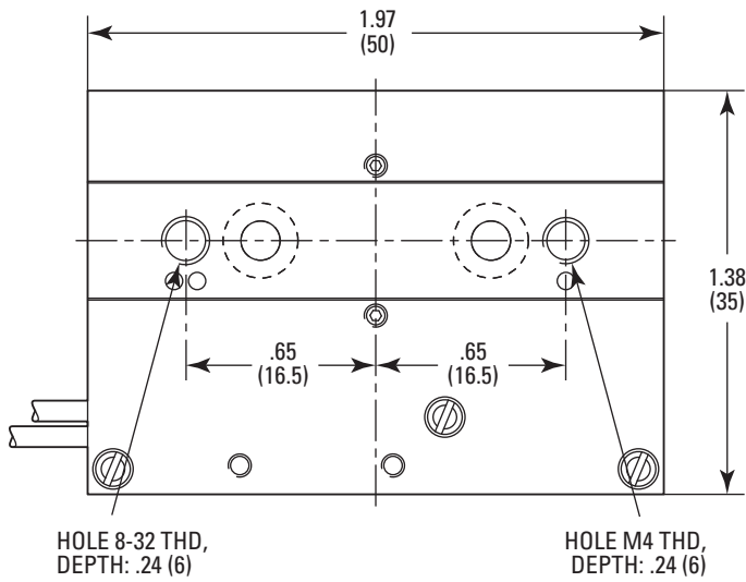
MODEL SHOWN: AG-LS25-27 DIMENSIONS IN INCHES (AND MILLIMETERS)
