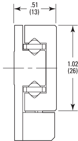
MODEL SHOWN: AG-LS25-27 DIMENSIONS IN INCHES (AND MILLIMETERS)
